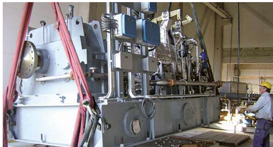
above_ Reduction gear right_ Turbine reducer module
